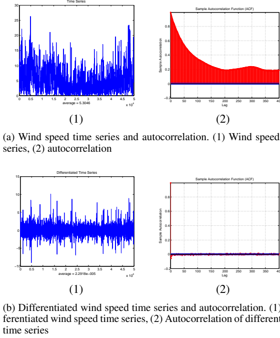
Figure 1: Autocorrelation analysis for time series wind speed data.
